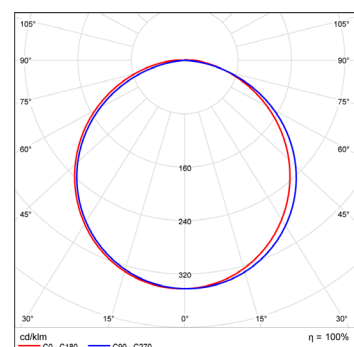
Polar curve for 1340 lumen LED strip with opal diffuser.
