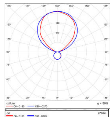
Polar curve for 3x1340 lumen LED strips with clear diffuser up and opal down.
