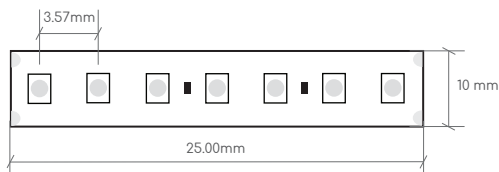
IP20 dimensions: W10 x H1mm
