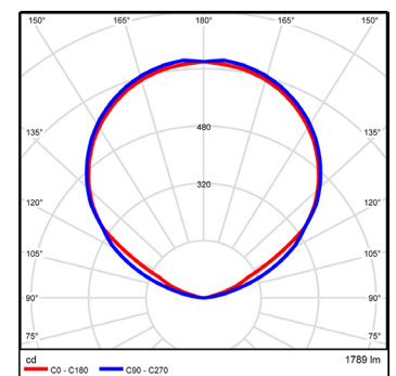
Polar curve for 3200 lumen LED strip with clear diffuser.
