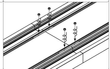
FIG. 3 - TIGHTEN SCREWS IN JOINER/BEND PLATES
