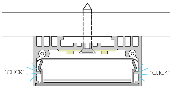
FIG. 4 - ENSURE DIFFUSER IS MOUNTED SECURELY
