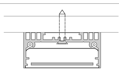
FIG. 3 - ENSURE EXTRUSION IS MOUNTED SECURELY
