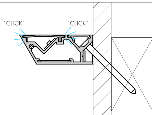
FIG. 2 - ENSURE DIFFUSER IS MOUNTED SECURELY
